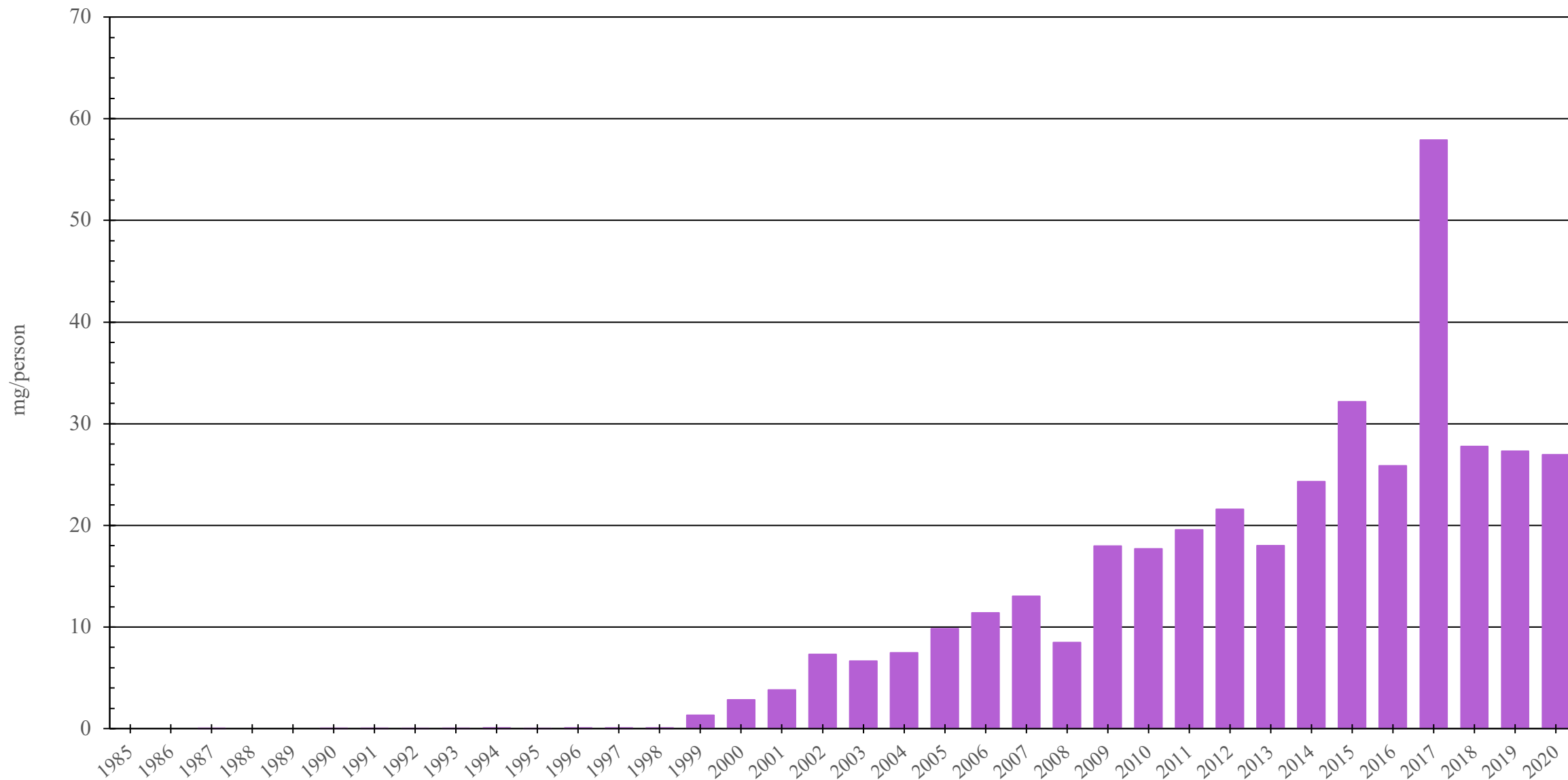
Oxycodone Consumption (mg/person), 1985 - 2020
